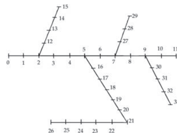
Figure 2. IEEE 34-bus distribution network test system [19].
