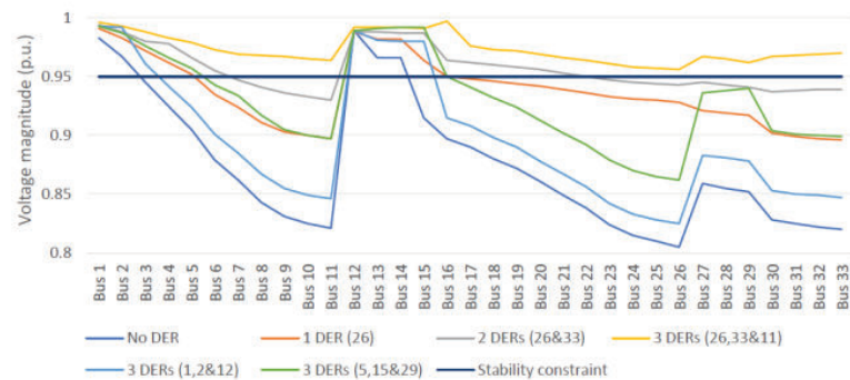
Figure 7. Voltage profile improvement with DER units placement.
