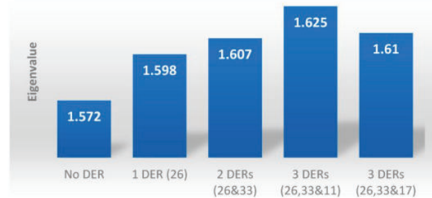
Figure 14. System eigenvalues with the CPF approach and the proposed method.
