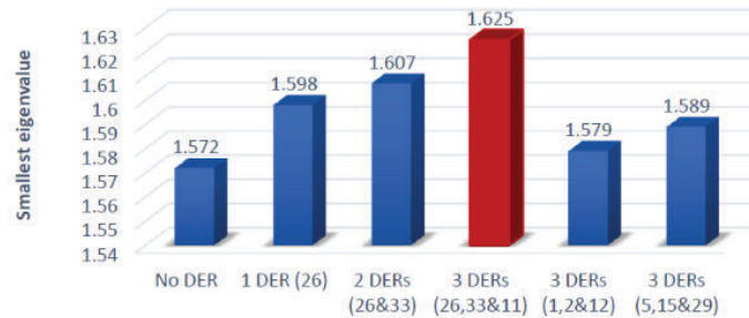
Figure 8. The system's smallest eigenvalue comparison.
