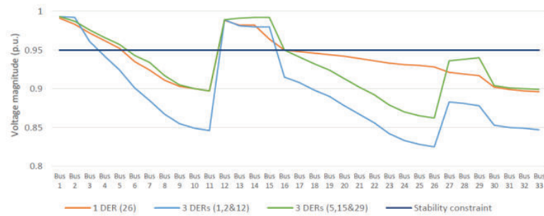
Figure 10. Comparison of voltage profile.
