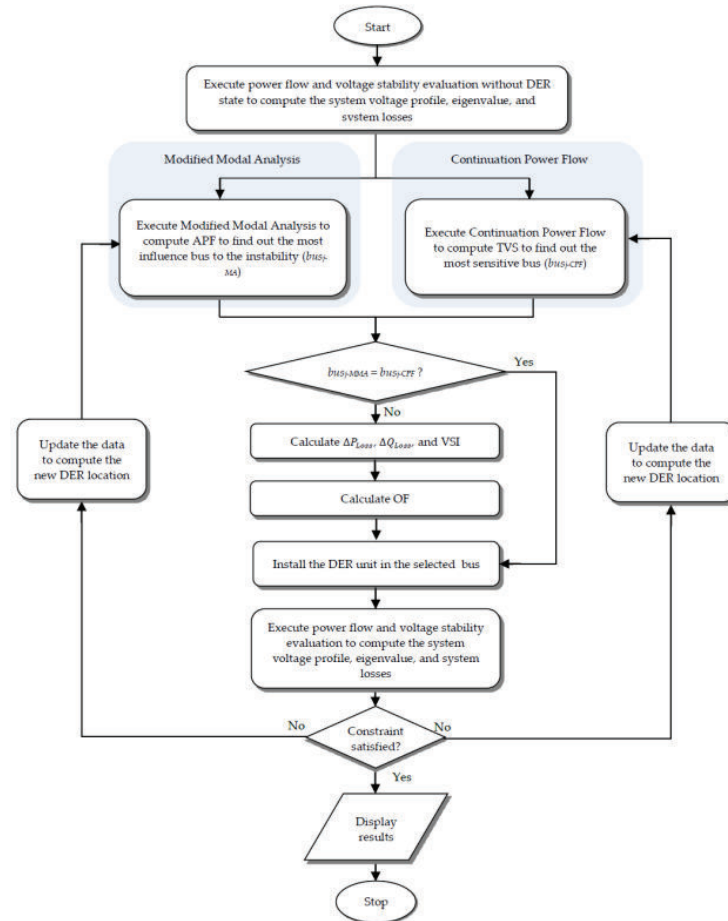
Figure 1. The hybrid MMA-CPF DER allocation approach flowchart.
